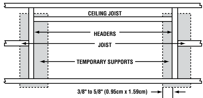
FIGURE 1 - FRAMED OPENING WITH TEMPORARY SUPPORT SLATS READY TO RECEIVE STAIRS
