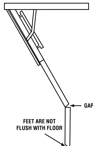
FIGURE 5C - INCORRECT SETUP
