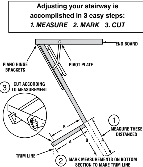
FIGURE 4A - ADJUSTMENT TO CEILING HEIGHTS
