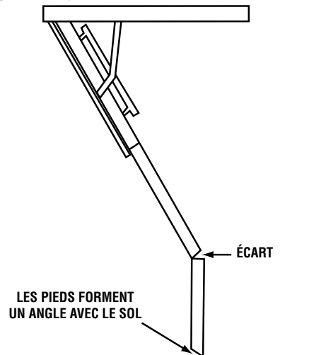
FIGURE 5C - MAUVAISE INSTALLATION
