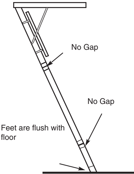
Correct Setup
